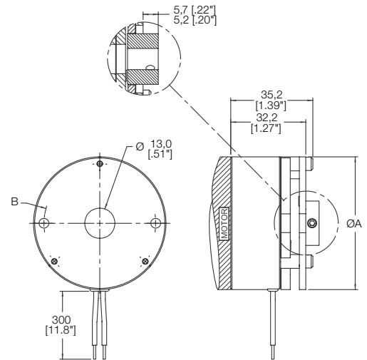
Magnet Mount
