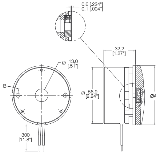
Flange Mount
