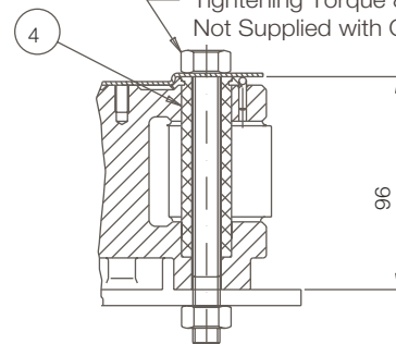
PART SECTION 'X-X'
