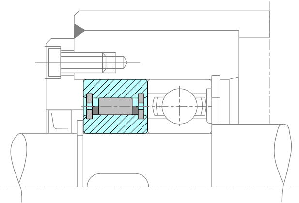
Figure 3: Mounting AS
