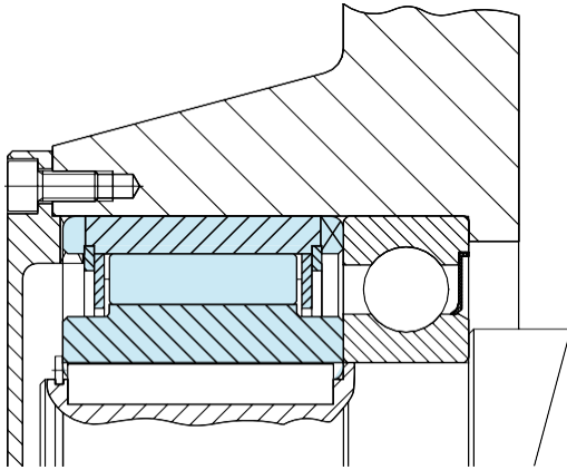
Figure 3: Mounting NF
