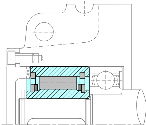
Fig. 4: Mounting AE
