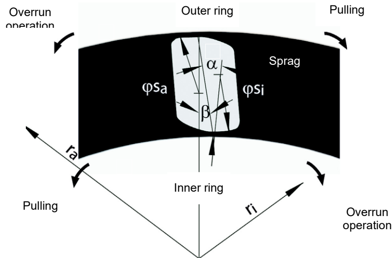
Fig. 2 Pulling/Overrun operation
