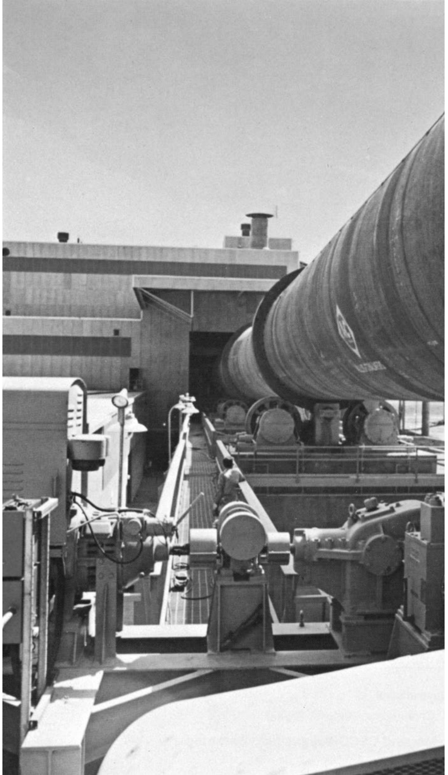
Photo: Marland CECON clutch and CEBMAG Backstop on modern cement kiln provide for emergency drive rotation in case of main power shutdown.
