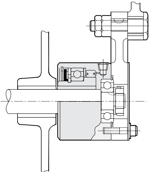
Indexing Clutch
